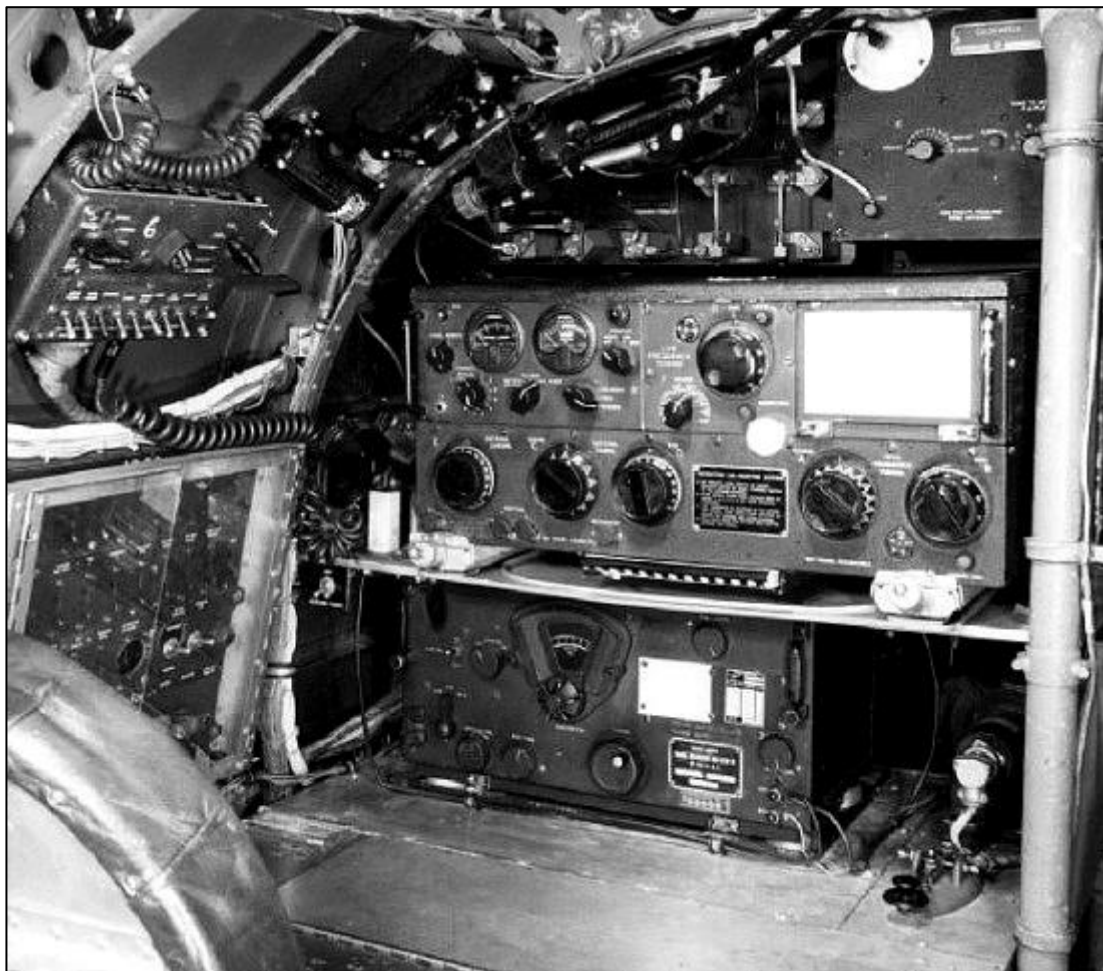
The ART-13 along with a BC-348 receiver installation onboard a Lancaster bomber.
